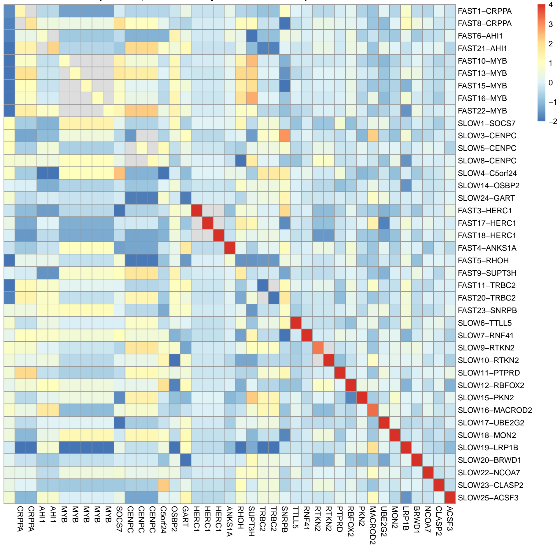
Clone Expression, Normalized by TPM and Gene Expression Last Exon
