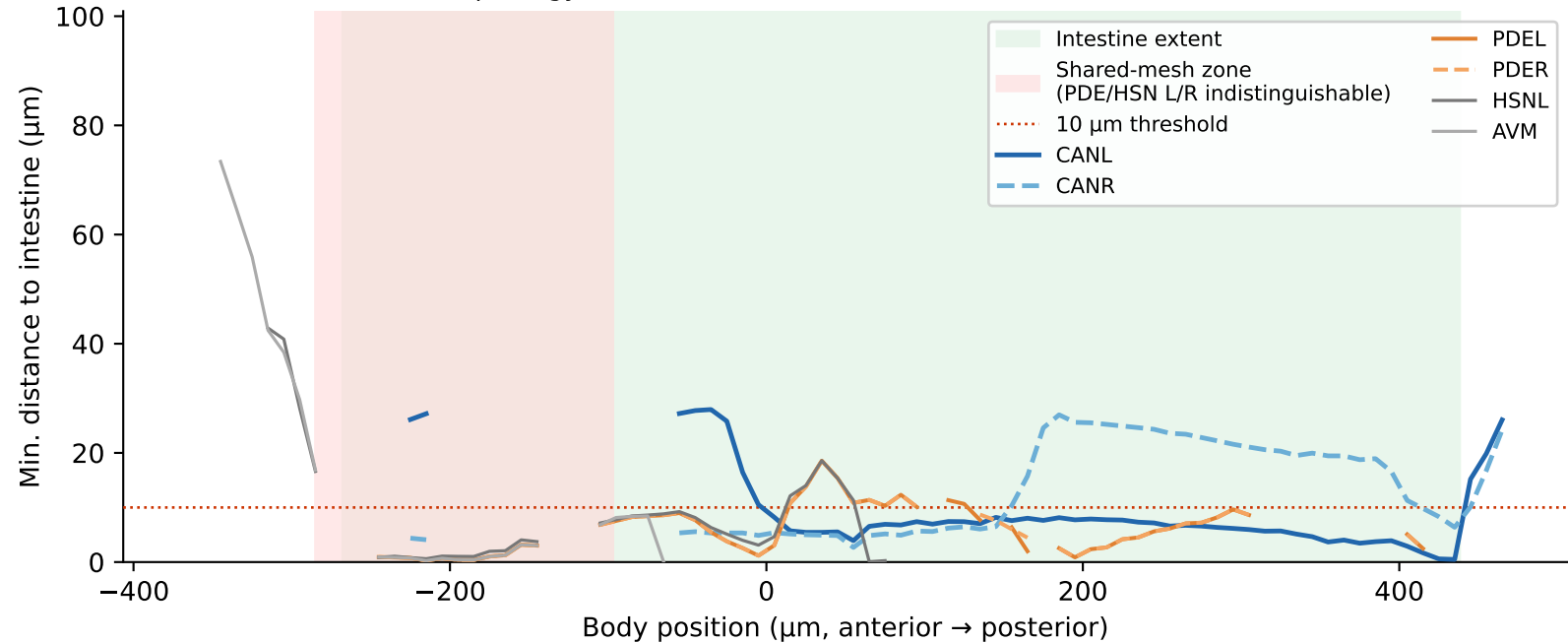
Neurite proximity to intestine along body axis (Virtual Worm Blender morphology, Blender-native coordinates)
