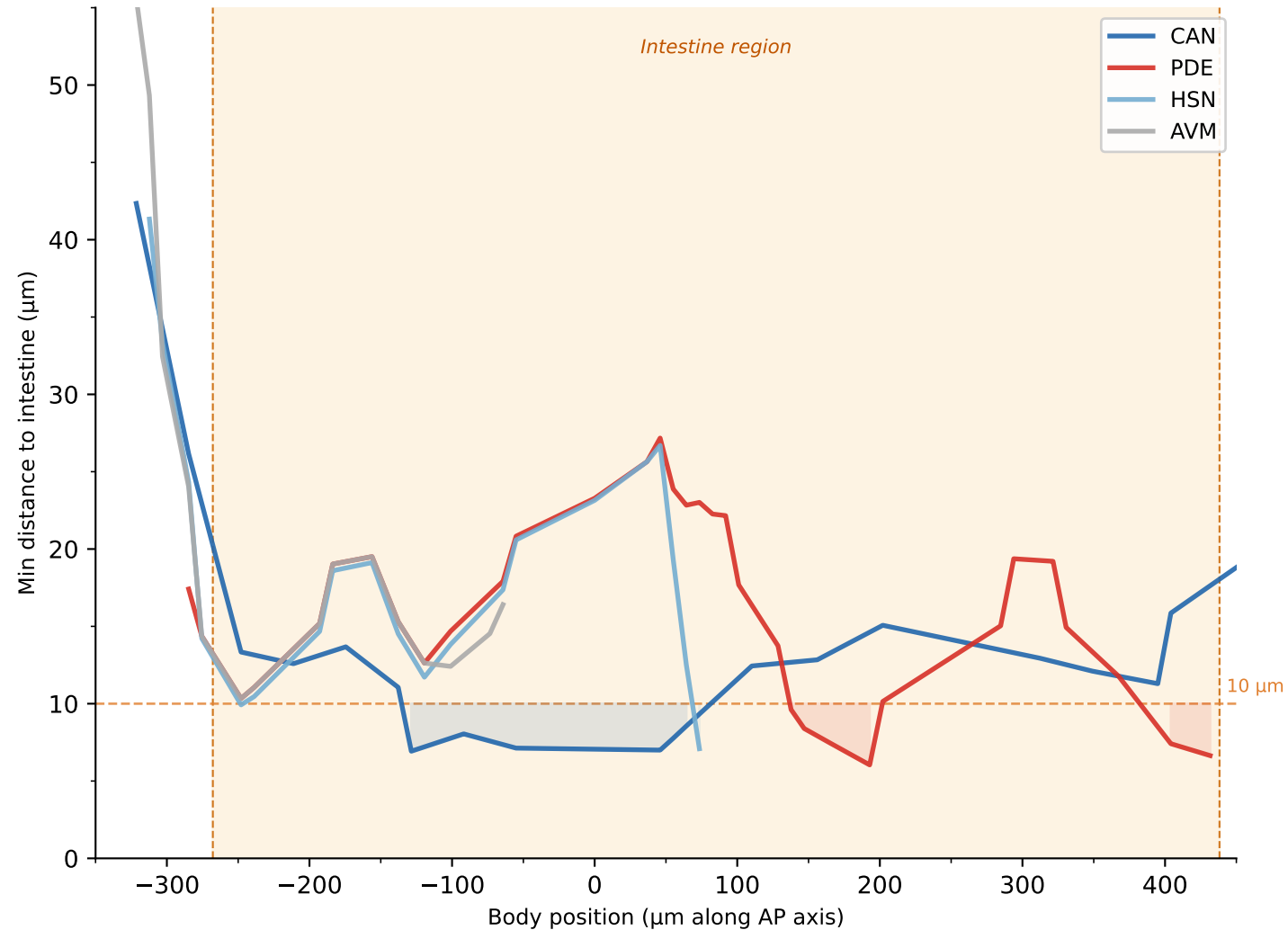
B Proximity along AP axis (min per ~9 μm body-axis bin, smoothed ×3)
