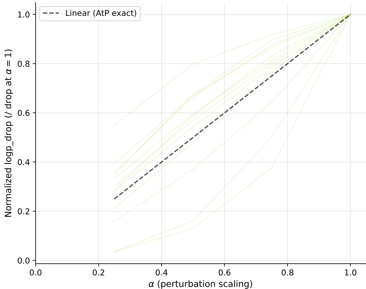
Layer 11: response curves (12 pairs)
