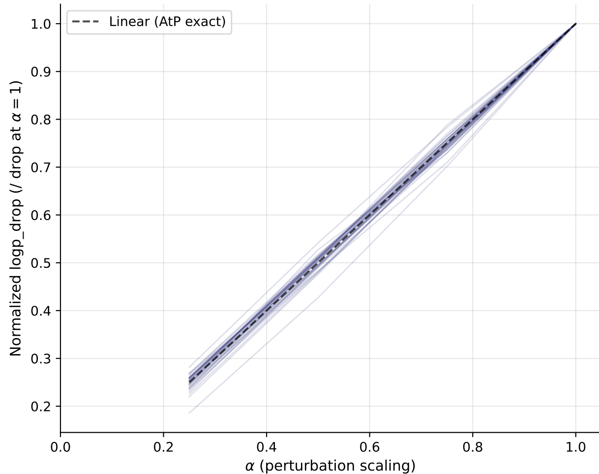
Layer 7: response curves (36 pairs)
