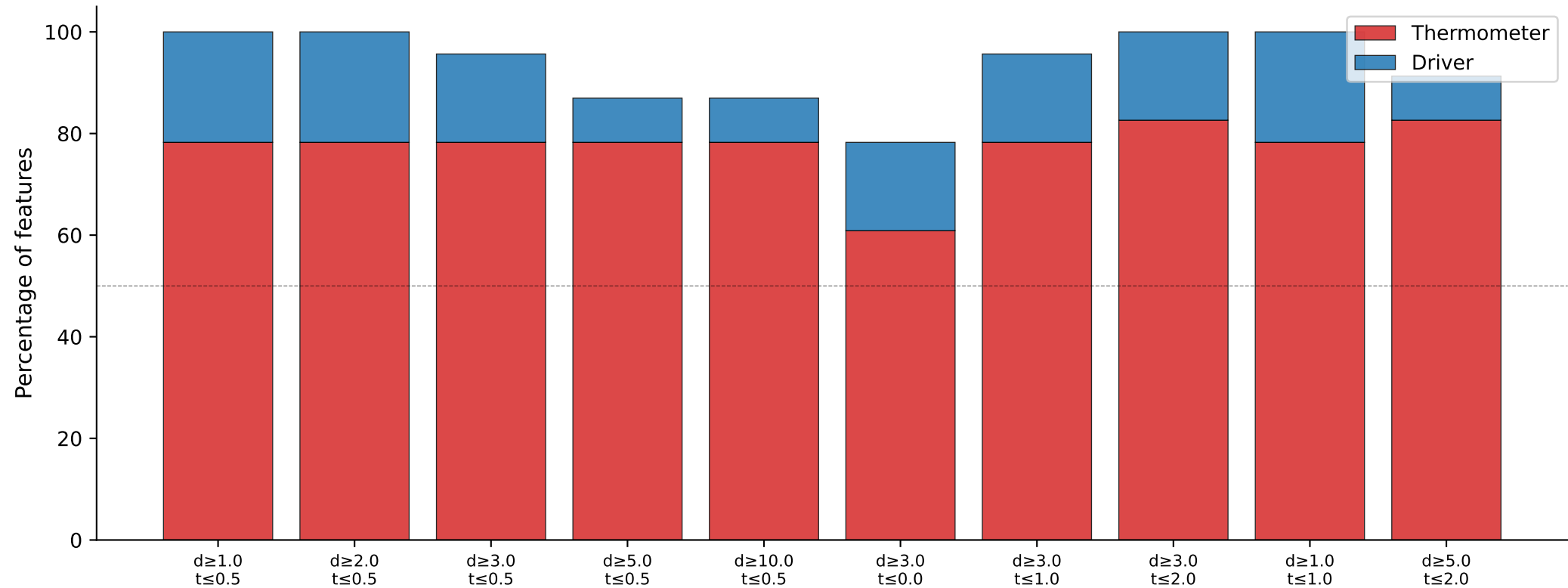
Threshold sensitivity: thermometer-majority is robust across 10 threshold pairs
