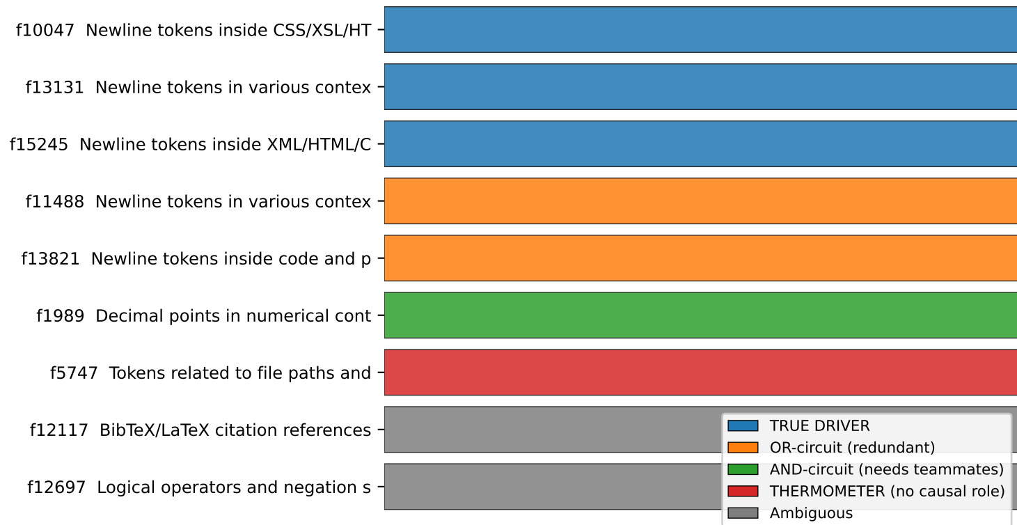
Per-feature classification
