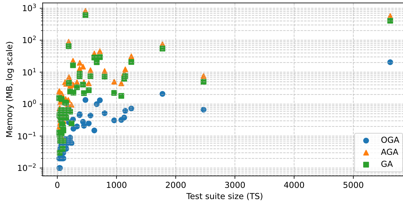
Memory vs Test-Suite Size
