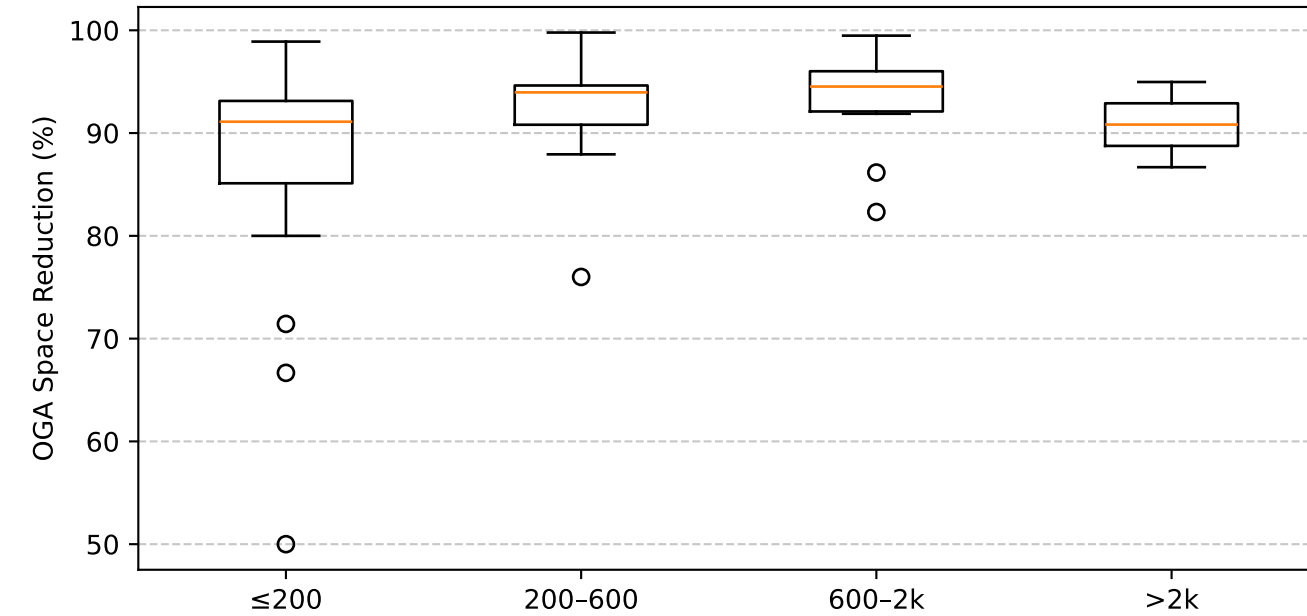
Space Reduction by Test-Suite Size
