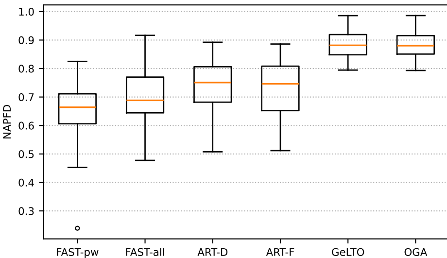
NAPFD (54 projects)
