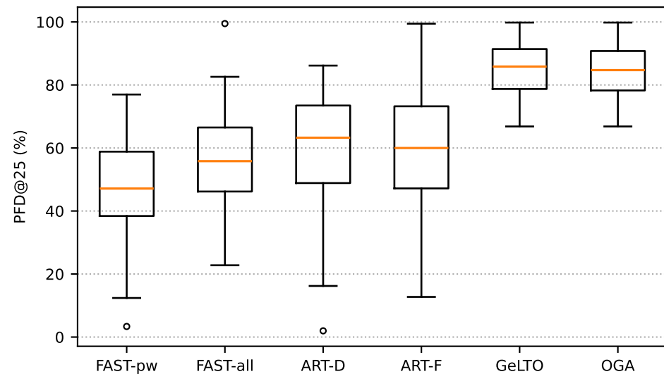
PFD@25 (54 projects)
