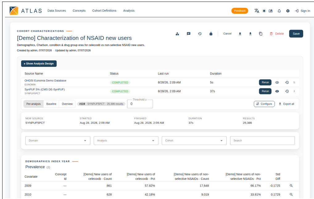
Figure 9.1. Characterization editor with the design hidden. The header shows the authorship line and the toolbar (including the Configure access lock); below it the data-source run table has a Rerun button, the eye View results icon, and the history icon with its run count per source, followed by the Per-analysis / Baseline / Overview toggle and the Domain / Analysis / Cohort / Search filter strip.
