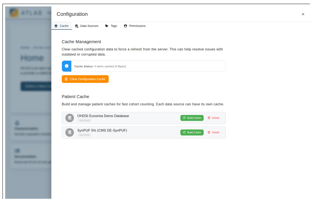
Figure 15.1. Configuration panel on the Cache tab (as an administrator sees it). The Cache Management card is at the top; the Patient Cache card below has a per-source row with the cache state (here Not Built ) and a Build Cache action.
