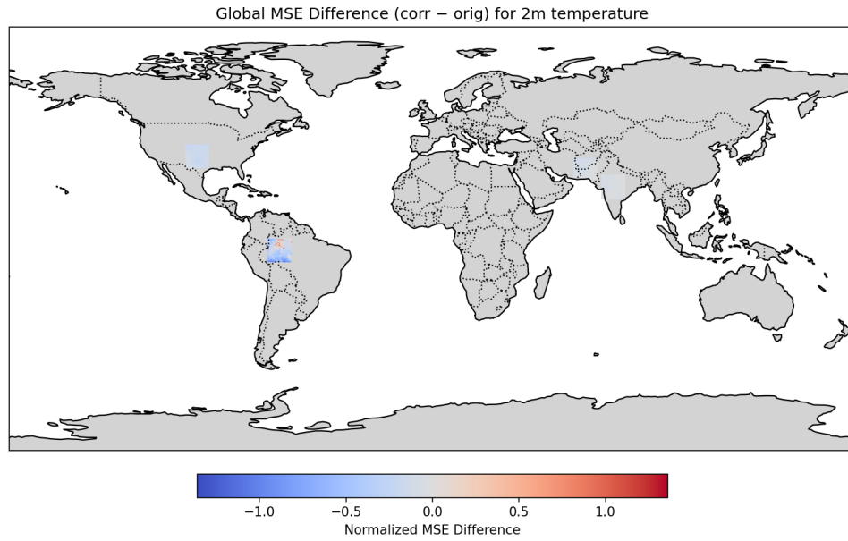
Figure 11: Global MSE comparison for 2m temperature: original vs corrected forecasts.
