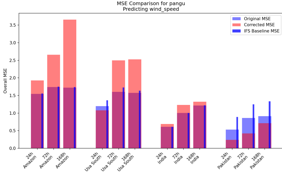
Figure 2: Overall MSE comparison for 10 m wind speed: original vs corrected forecasts.
