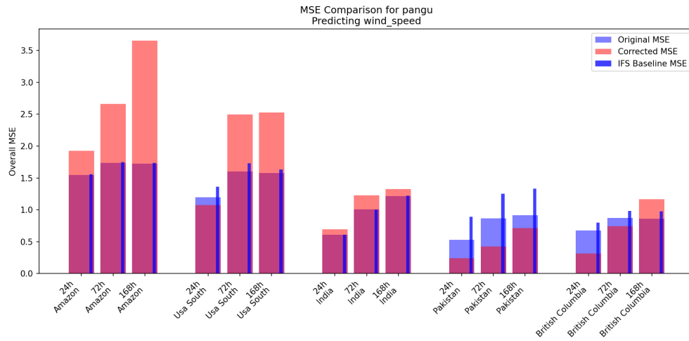
Figure 2: Overall MSE comparison for 10m wind speed: original vs corrected forecasts.
