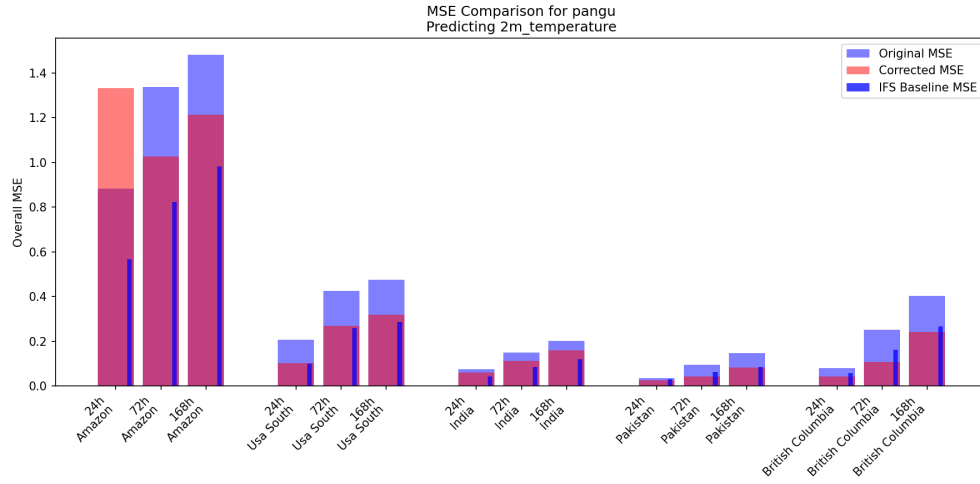
Figure 1: Overall MSE comparison for 2m temperature: original vs corrected forecasts.
