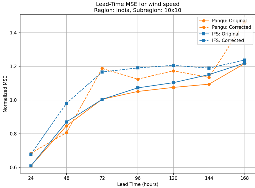
Figure 4: 10m Wind Speed MSE comparison for forecasts trained on different lead times.
