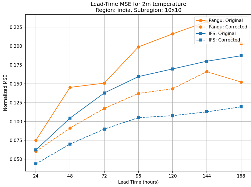
Figure 3: 2m Temperature MSE comparison for forecasts trained on different lead times.
