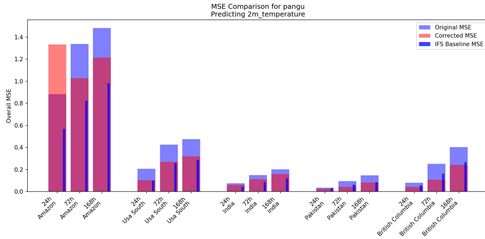
Figure 1: Overall MSE comparison for 2 m temperature
