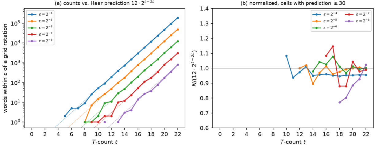
Figure 1: Number of Clifford+ T words of T -count exactly t within \epsilon of a grid rotation on a Haar-random coset G_1 R_z(\theta) G_2 . (a) Counts (markers) against the Haar prediction 12 \cdot 2^{t-2L} (dashed). (b) The same counts divided by that prediction, plotted where the prediction is at least 30; every \epsilon has reached the Haar value by t = 22 . Exhaustive enumeration to t = 22 ( 1.5 \times 10^8 words).
