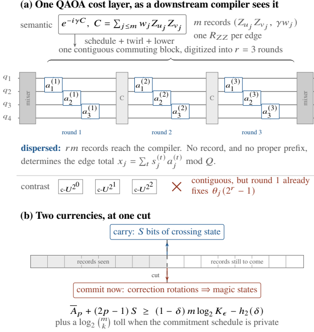
FIG. 1. Dispersal, and the two currencies that undo it. (a) A QAOA cost layer e^{-i\gamma C} on m edges is one commuting object carrying m records. Lowered under a digitized schedule it reaches a downstream compiler as r contiguous rounds of grid residues, optionally sign-randomized and separated by Clifford records; the edge total x_j is then a sum that no single record and no proper prefix reveals. The mixer layers bound the block rather than sitting inside it: at generic angles they are non-Clifford R_X rotations (remark 10). The controlled-power ladder beneath is the complementary case—its rounds are contiguous, but round one already fixes the aggregate \theta_j(2^r - 1) , so it supplies contiguity without dispersal (remark 7). (b) At any cut the scattered information is either carried across in compiler state or committed to output and repaid downstream in magic states. Theorem 5 states that the two cannot both be small, and proposition 7 charges the committed channel a further \log_2 \binom{m}{k} when the commitment schedule is private.
