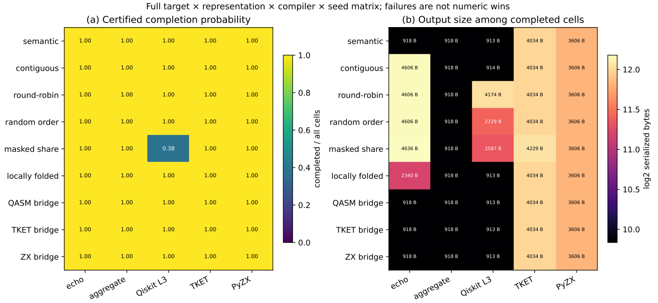
FIG. 4. Complete matched-representation interaction summary. Panel (a) reports certified completion probability for every representation–compiler pair; panel (b) reports serialized output size only among completed cells. Predicate errors remain status observations and never become numerical wins.
