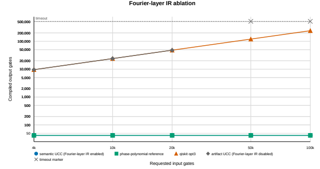
FIG. 8. Mechanism ablation for the fixed-width HD^rH witness. Disabling the Fourier-layer semantic path yields completed but linearly large outputs through 20k and timeout rows at 50k and 100k, while Fourier-enabled semantic UCC and the phase-polynomial reference recover the canonical 42-gate circuit.
