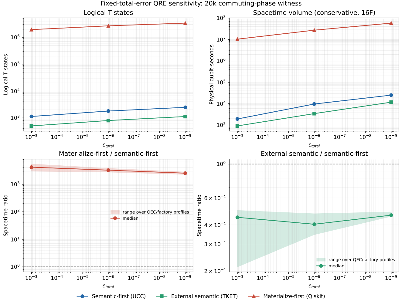
FIG. 13. Sensitivity to total error, QEC profile, and factory count on the 20k witness. Top: logical T demand and the conservative-profile spacetime volume. Bottom: ratios to semantic-first, with bands spanning both QEC profiles and all four factory counts. The dashed line is equality. No materialize-first reversal occurs in the measured grid; the strong external TKET path is reported on the semantic-capable side.
