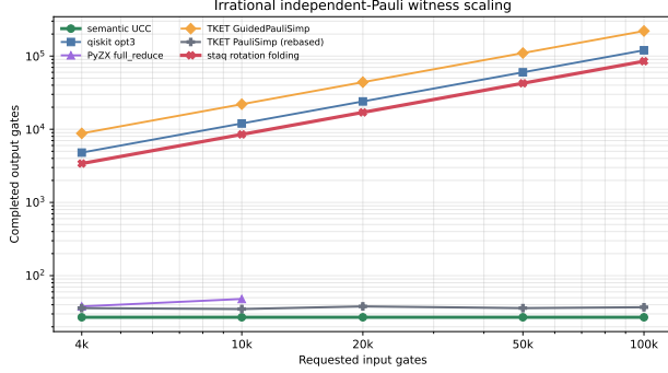
FIG. 7. Configured-pipeline scaling on the irrational independent-Pauli witness. Semantic UCC remains at 27 gates. Rebased TKET PauliSimp returns a small validated form at all five scales, demonstrating that a generic pipeline can cross the formal boundary by reconstructing an aggregate Pauli representation. Public staq rotation folding, qiskit opt3 , and TKET GuidedPauliSimp grow with input size. PyZX full_reduce completes at 4k and 10k, fails the numerical tolerance at 20k, and reaches the time budget at larger scales. Status-only cells are omitted from numerical curves.
