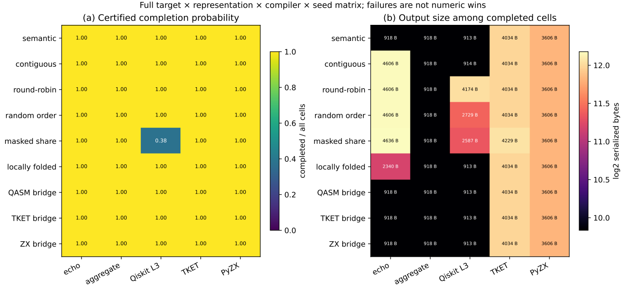
FIG. 4. Complete matched-representation interaction summary. Panel (a) reports certified completion probability for every representation–compiler pair; panel (b) reports serialized output size only among completed cells. Predicate errors remain status observations and never become numerical wins.
