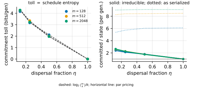
FIG. 3. The commitment toll, preregistered and measured on the two-round masked-share device; every cell restart-verified. Left: bits per committed generator paid by a self-identifying committed prefix in excess of the deferred snapshot, against the predicted schedule entropy \log_2 \binom{m}{k} / k (dashed). The toll is flat in m and vanishes at \eta = 1 . Right: the per-generator exchange rate between the committed and state channels. Solid: irreducible, under an identity-optimal serializer—at most 2.64, and exactly 1 when the commitment schedule is public. Dotted: the same rate as actually serialized by the address-per-record codec of figure 2, which is where the 6:1 comes from and which is the only part that grows with address width. Frozen artifact: generated/e8_commit_toll.json , generated by PaperDraft/scripts/run_commit_toll.py .
