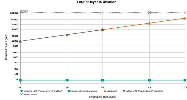
FIG. 8. Mechanism ablation for the fixed-width HD^rH witness. Disabling the Fourier-layer semantic path yields completed but linearly large outputs through 20k and timeout rows at 50k and 100k, while Fourier-enabled semantic UCC and the phase-polynomial reference recover the canonical 42-gate circuit.
