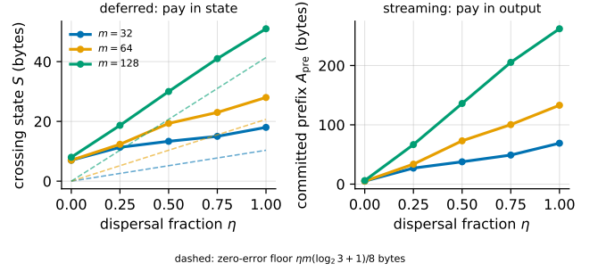
FIG. 2. Measured dispersal–memory tradeoff on the executable two-round masked-share device ( Q = 3 , binary aggregates, tracked signs; every point restart-verified: the serialized snapshot alone plus the round-two suffix reproduces the exact output). Left: a deferred compact-output compiler pays the dispersal in crossing state; measured slopes 10.3/21.1/43.3 bytes per unit \eta at m = 32/64/128 sit on the zero-error floor \eta m(\log_2 3 + 1)/8 bytes (dashed; ratios 0.99–1.05), the residue-plus-frame cost of theorem 4 and proposition 5. Right: a streaming compiler pays the same dispersal in committed prefix output ( A_{\text{pre}} slopes 60/129/260 bytes per unit \eta , larger by the public addresses) while its crossing state stays flat at \leq 8 bytes. The horizontal axis is the dispersal fraction \eta of proposition 6. Frozen artifact: data/frozen/eta_sweep_pareto.json , generated by PaperDraft/scripts/run_eta_sweep.py .
