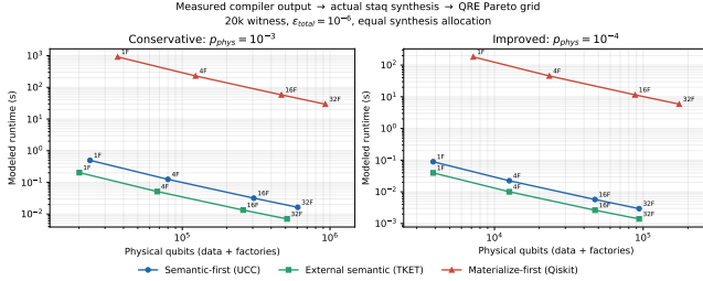
FIG. 9. Physical-qubit/runtime Pareto grid at the representative 20k, \epsilon_{\text{total}} = 10^{-6} slice. Labels give factory counts. The external TKET path receives a materialized CX- R_Z -H bridge but reconstructs a compact phase form before synthesis, so it is classified as semantic-capable.
