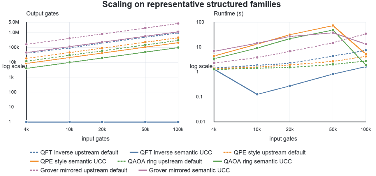
FIG. 14. Scaling behavior on representative structured families. Left: output gate count versus input gate count for upstream default (baseline UCC) and the semantic UCC artifact. Right: runtime versus input gate count. The semantic path preserves clear quality advantages across scale, while runtime behavior remains family-dependent.
