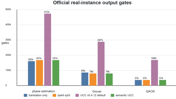
FIG. 10. Total output gate counts on the three official real instances. The semantic UCC artifact matches qiskit opt3 -level output quality while substantially improving over the upstream UCC v0.4.12 pre-semantic default.
