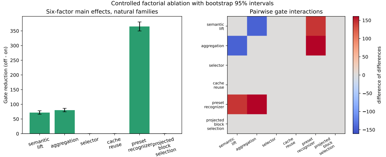
FIG. 12. All six factorial gate-count main effects and pairwise interactions. Zero-effect factors are displayed rather than omitted.
