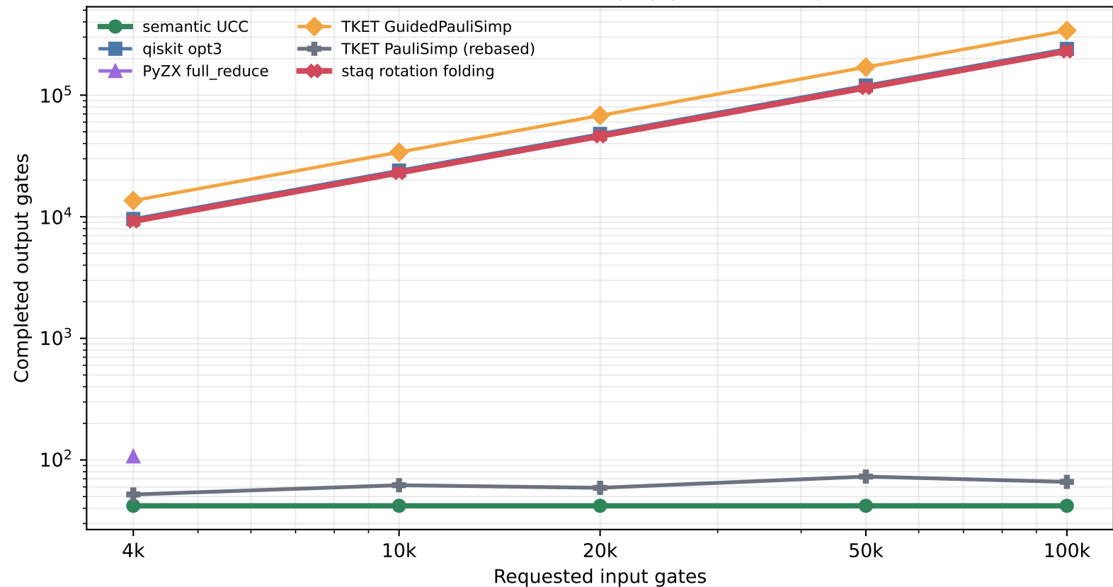
Rational CP finite-range pipeline scaling
