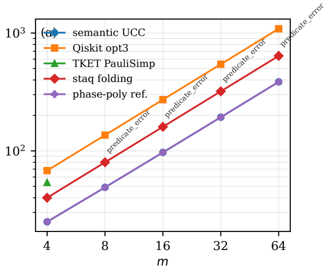
completed output gates
