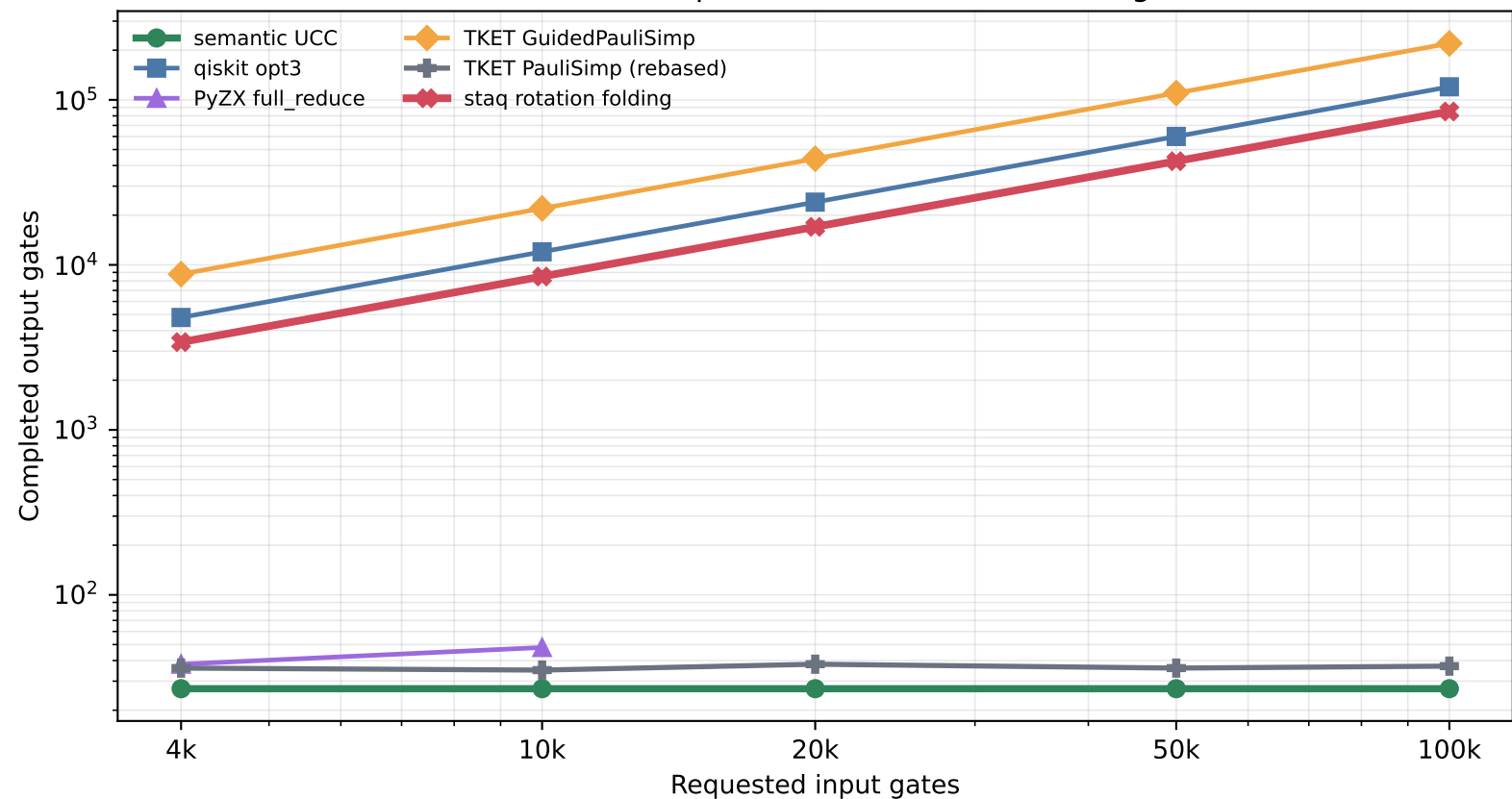
Irrational independent-Pauli witness scaling
