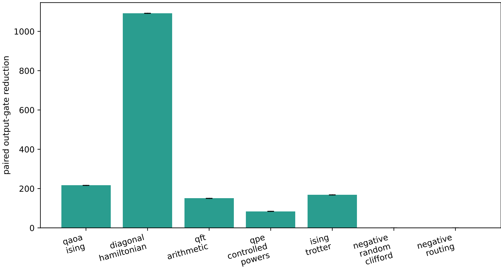
Semantic-lift effect with selector and preset disabled (95% CI)
