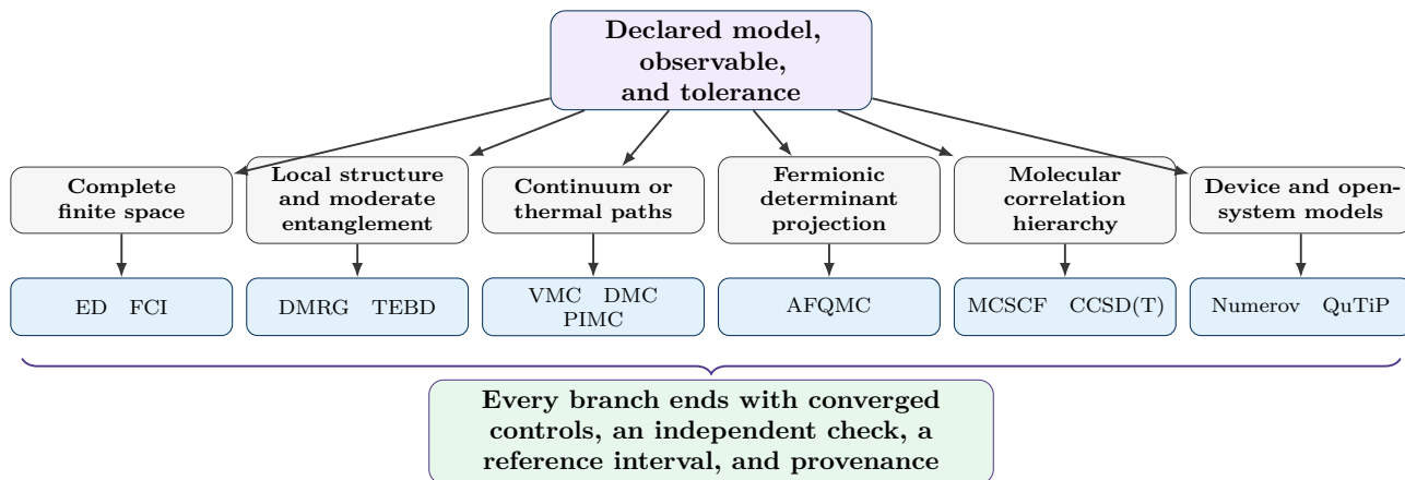
Figure 14.2: Branched solver map for constructing a numerical ground-truth record. The final reference interval still requires convergence and an independent check.
