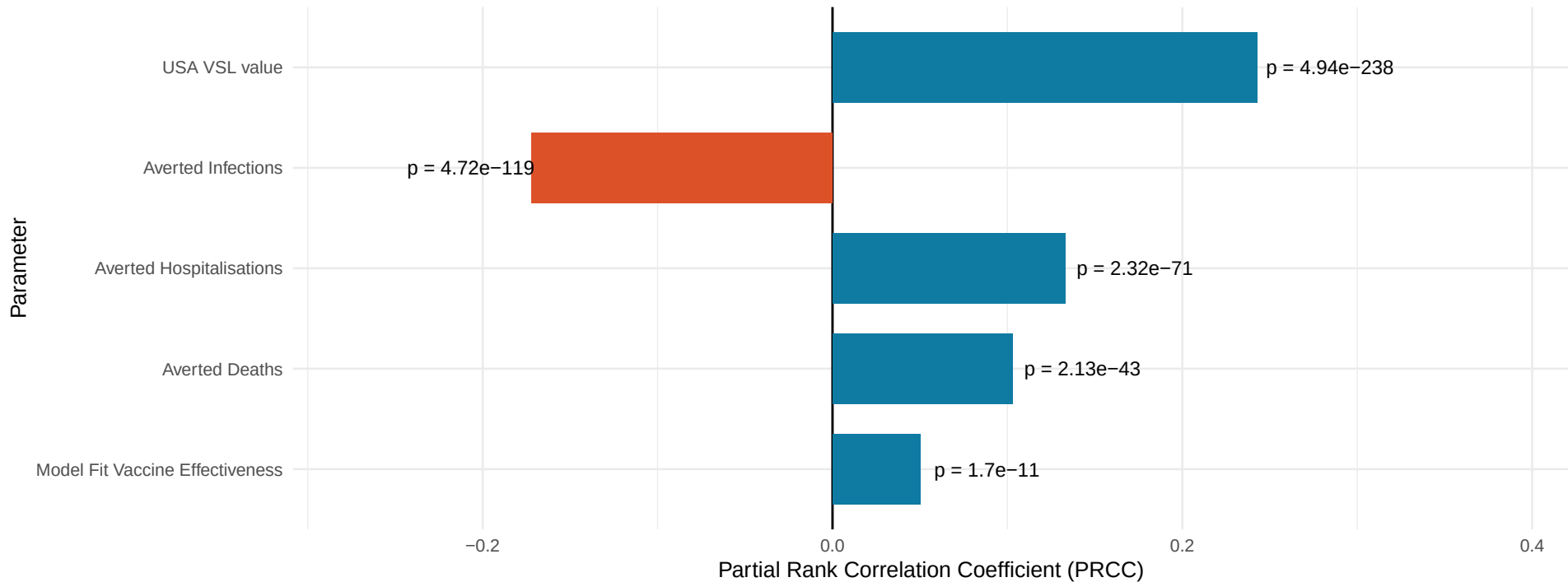
Tornado Plot of PRCC Values
