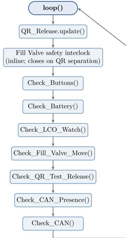
Figure 2: GSEMU main loop control flow.
