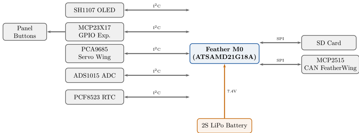
Figure 1: GSEMU hardware block diagram.
