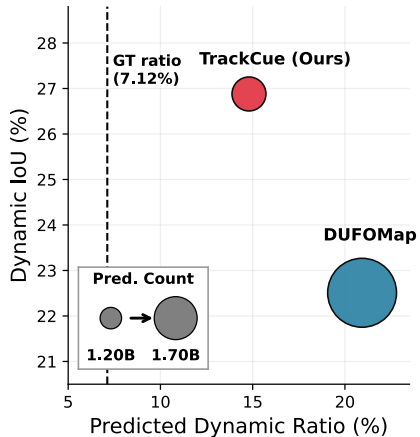
(a) Dynamic Ratio vs. Classification Quality
