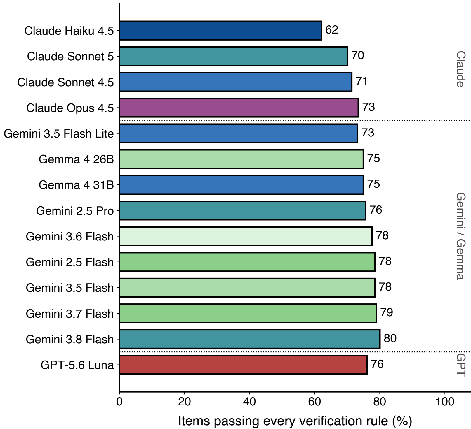
(a) Pass rate per translator
