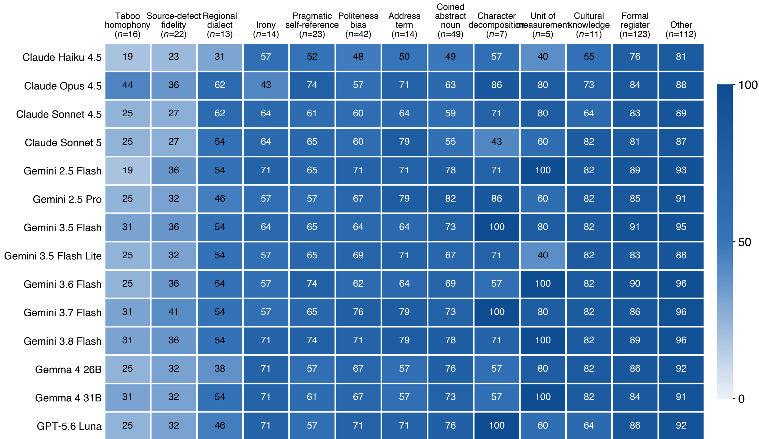
(b) Pass rate by mechanism family (%)
