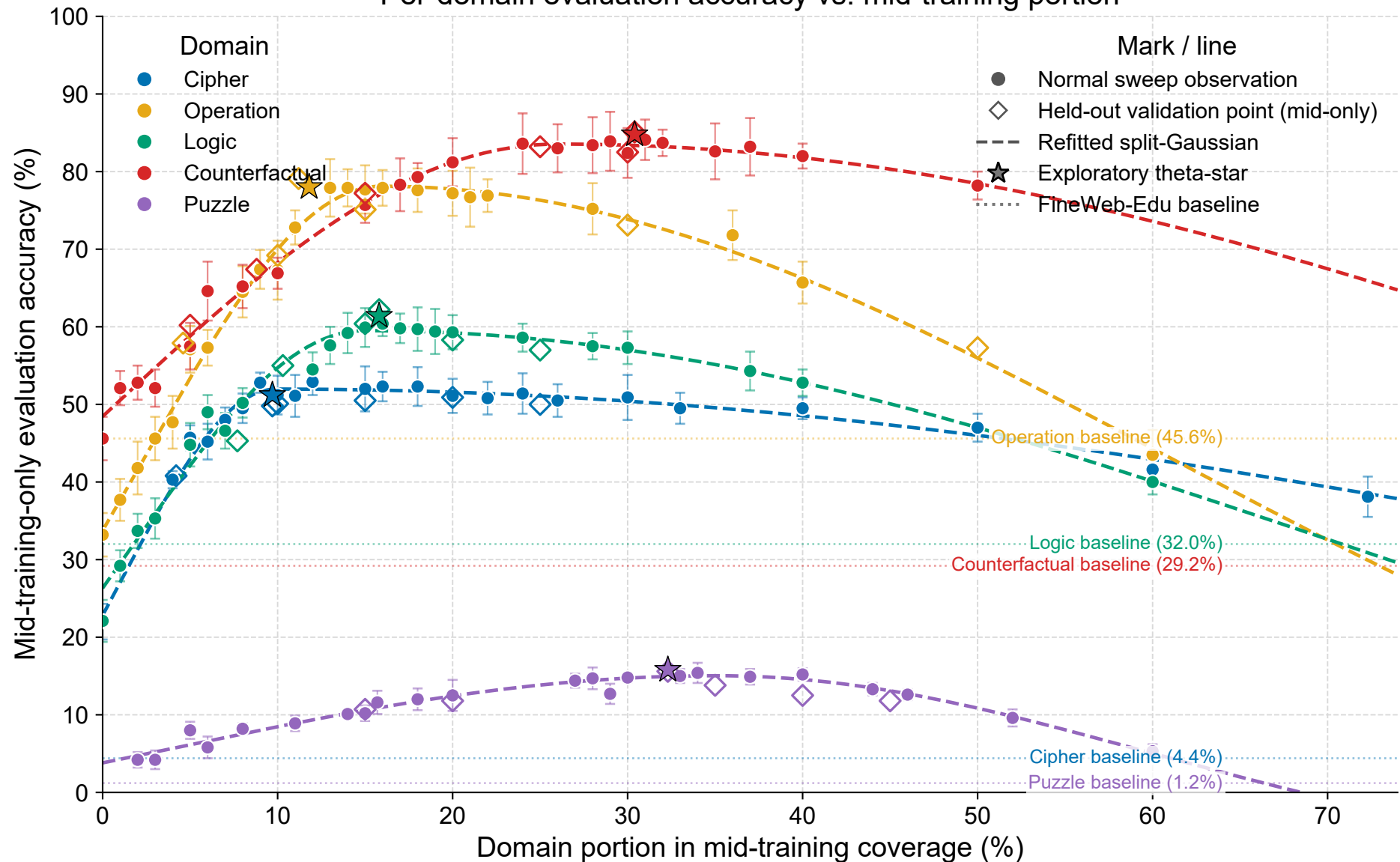
Per-domain evaluation accuracy vs. mid-training portion
