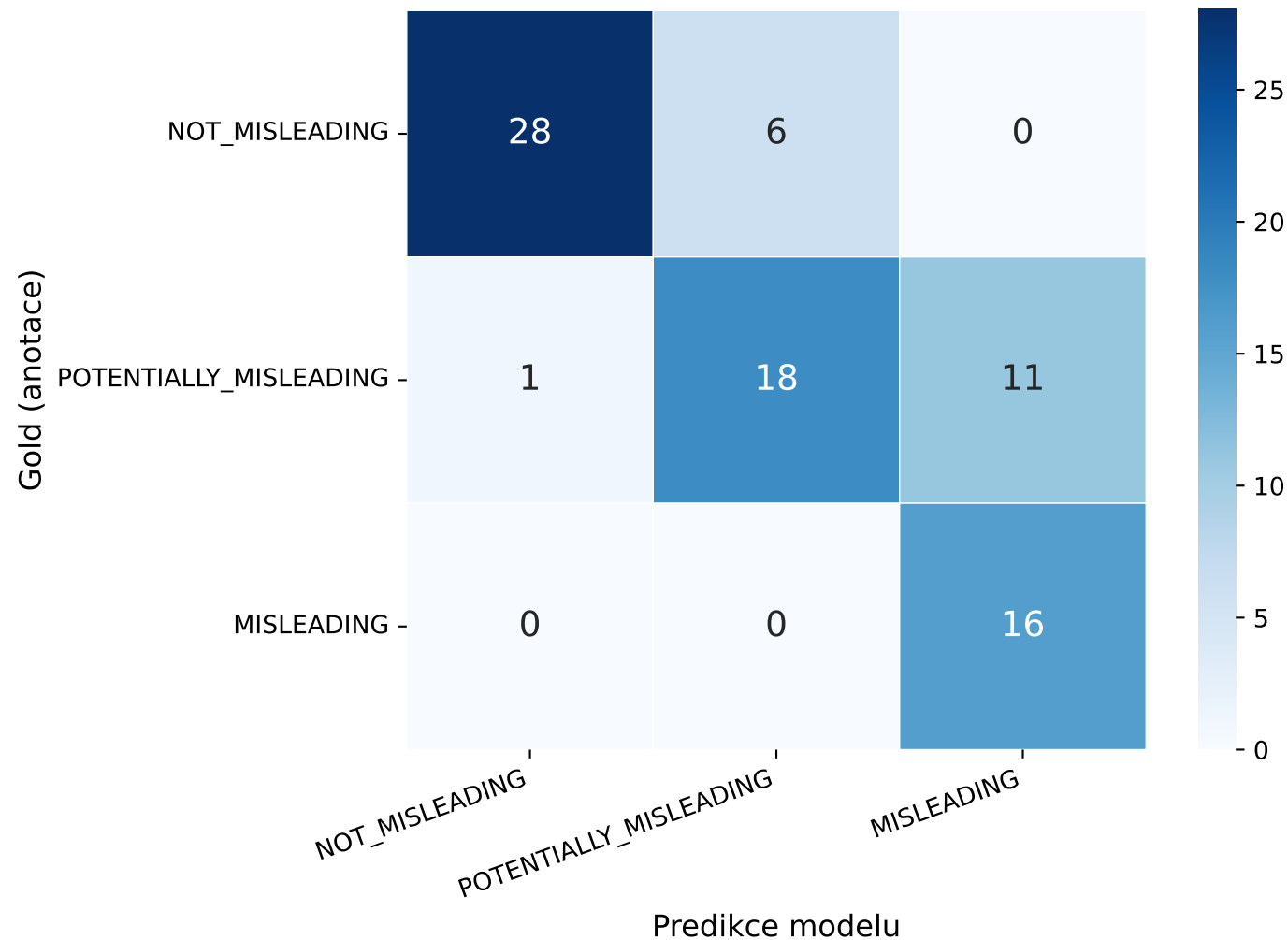
Confusion Matrix — gpt_5_5_zs E1-misleading_header_model_final
