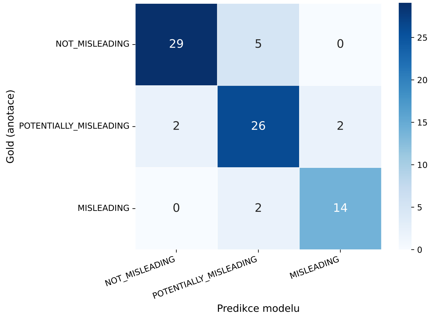
Confusion Matrix — gpt_5_5_zs_short E1-misleading_header_model_final
