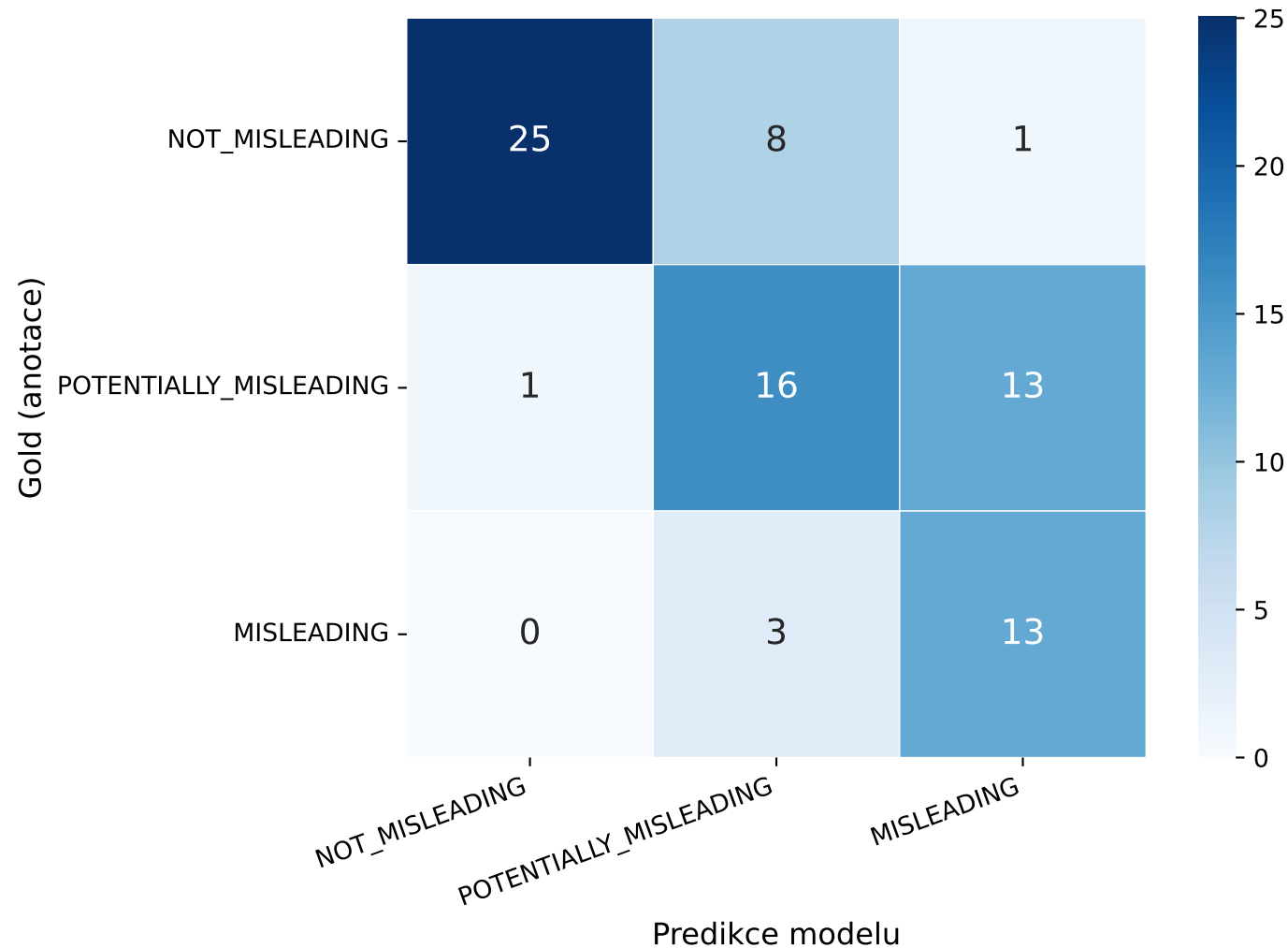
Confusion Matrix — llama_instruct_qlora_zs E1-misleading_header_model_final
