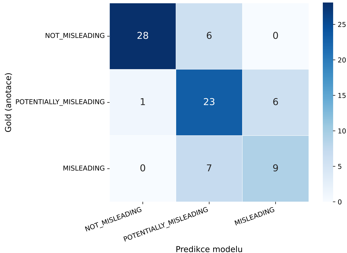
Confusion Matrix — llama_instruct_qlora_zs_short E1-misleading_header_model_final
