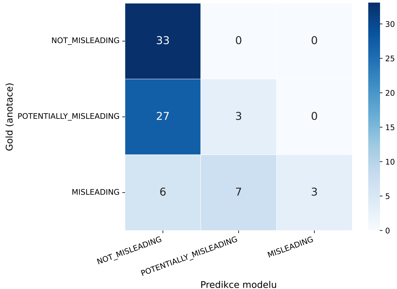
Confusion Matrix — llama_instruct_zs_short E1-misleading_header_model_final
