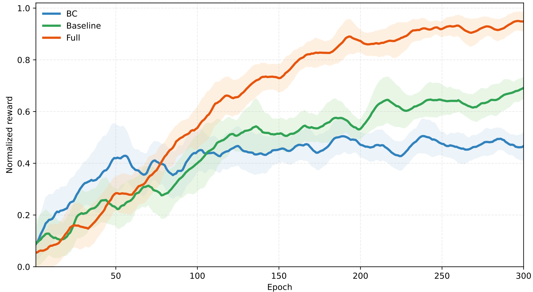
Offline Training Reward Curve with Mean \pm Std
