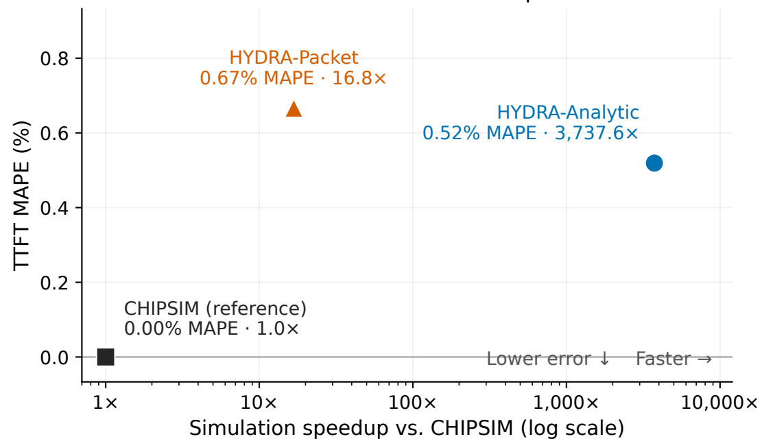
TTFT error vs. simulation speed
