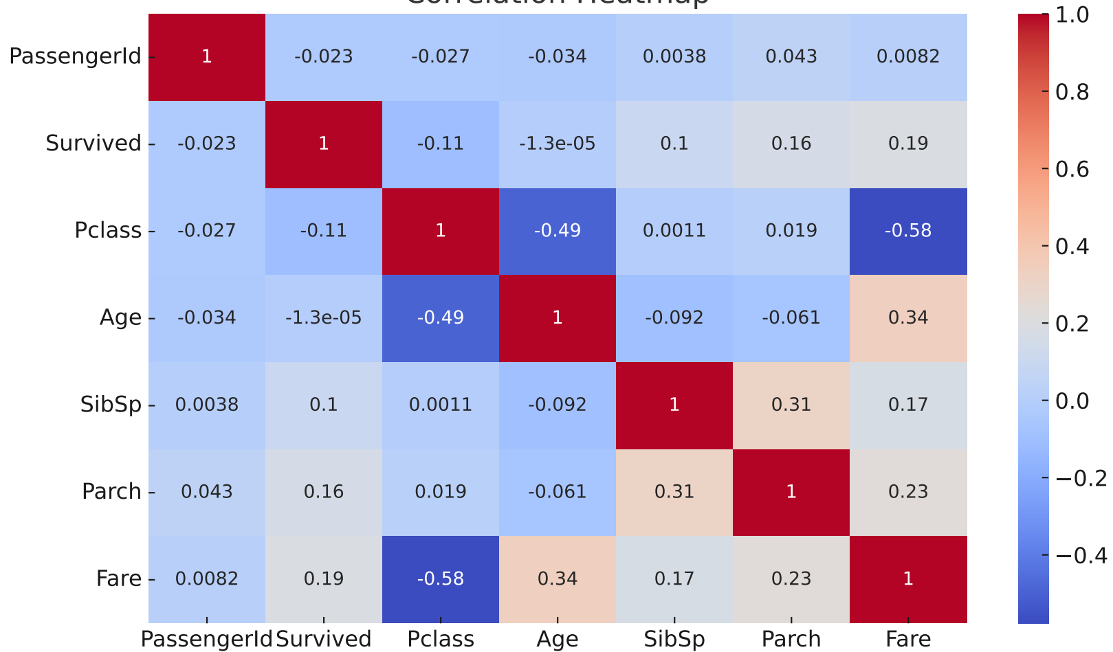
Correlation Heatmap
