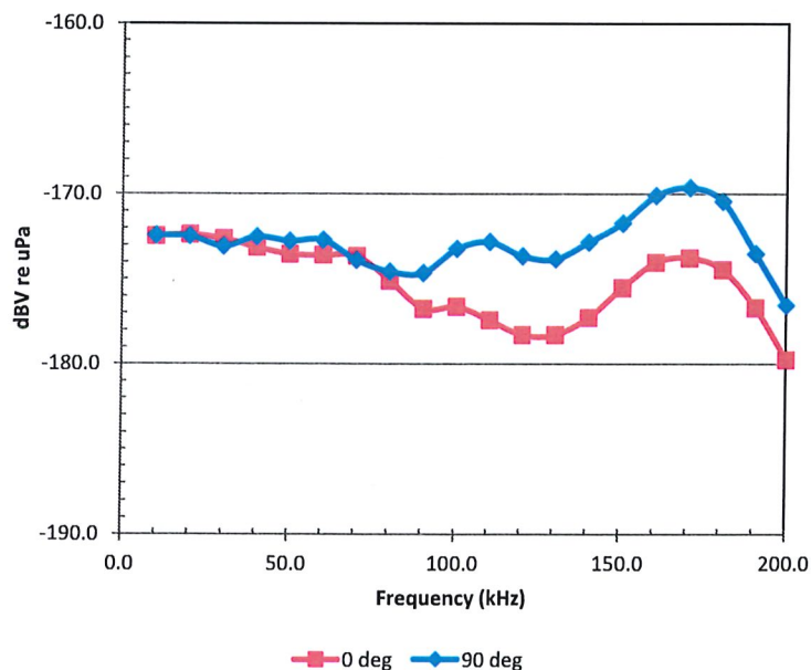
Receive Sensitivity
