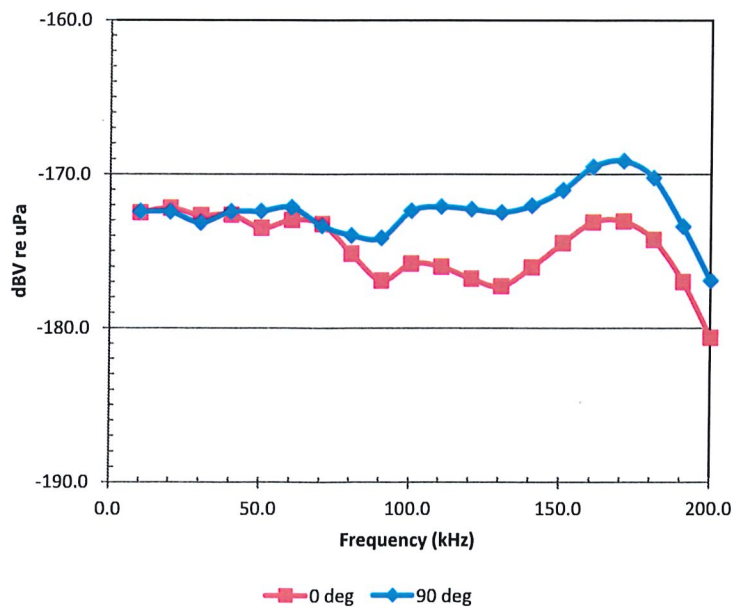
Receive Sensitivity
