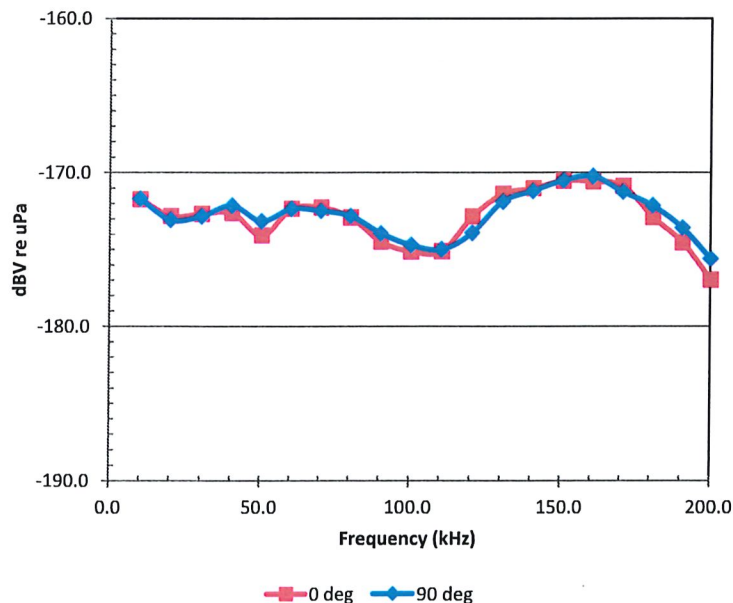
Receive Sensitivity
