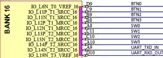
XC7A100T-1CSG324C
