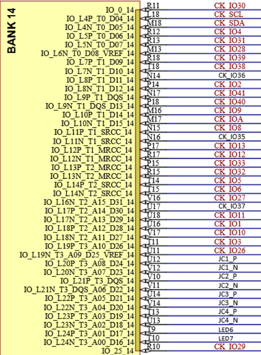
XC7A100T-1CSG324C
