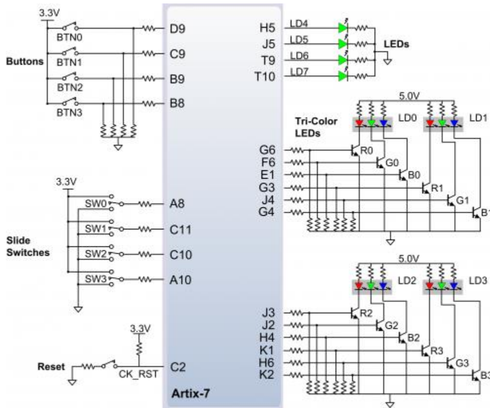
Figure 9.1. Arty GPIO.
