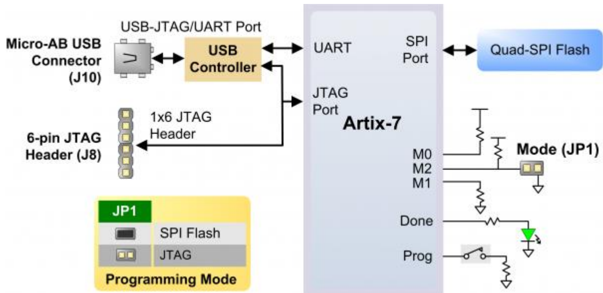
Figure 4.1. Arty configuration.
