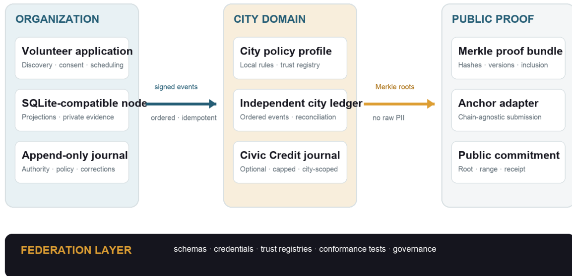
Figure 1. Target architecture. Private operational payloads remain within organization and city domains. Public chains receive only approved commitments and non-sensitive metadata.
