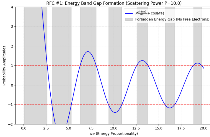
Figure 1: Phase 1: Proof of Forbidden Energy Zones where |\cos(ka)| > 1 .
