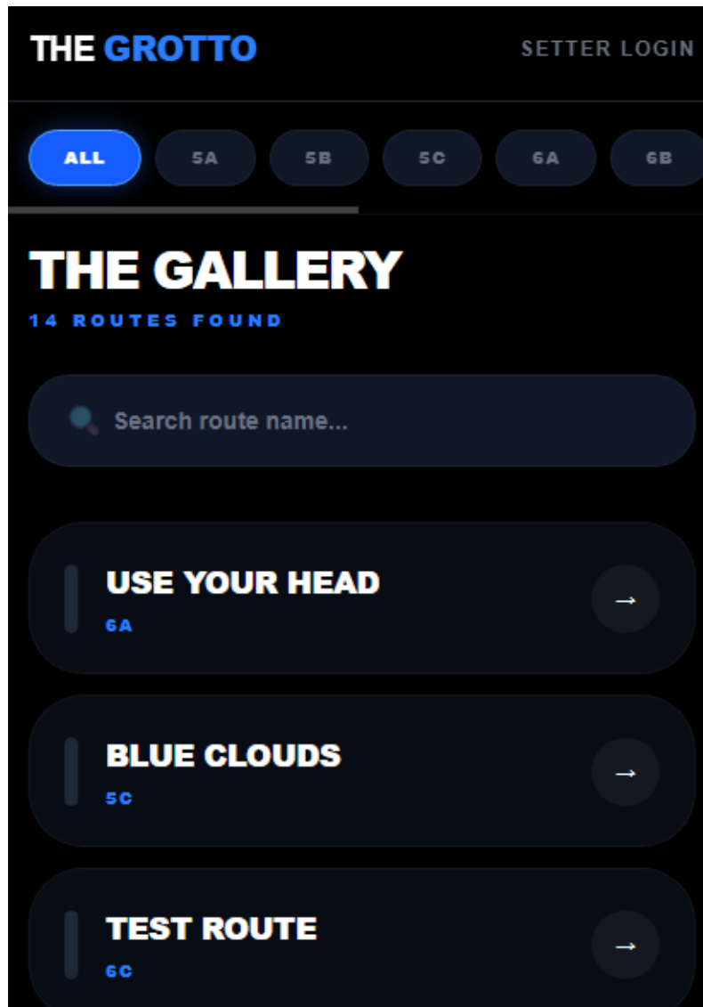
[IMAGE: Main Gallery] Screenshot of the home screen showing the horizontal grade filter bar and the route cards.
