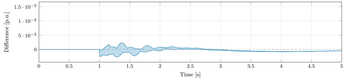
(c) EMT minus PhasorDynamics: range across channels
