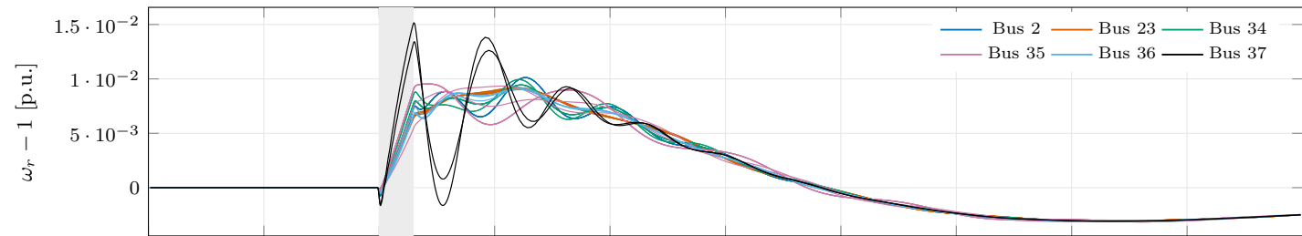
(b) GridKit PhasorDynamics; fault cleared at 1.15 s (30 machines)
