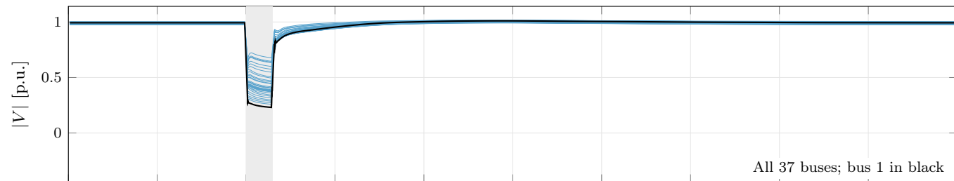
(b) GridKit PhasorDynamics; fault cleared at 1.15 s
