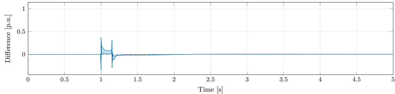
(c) EMT minus PhasorDynamics: range across channels
