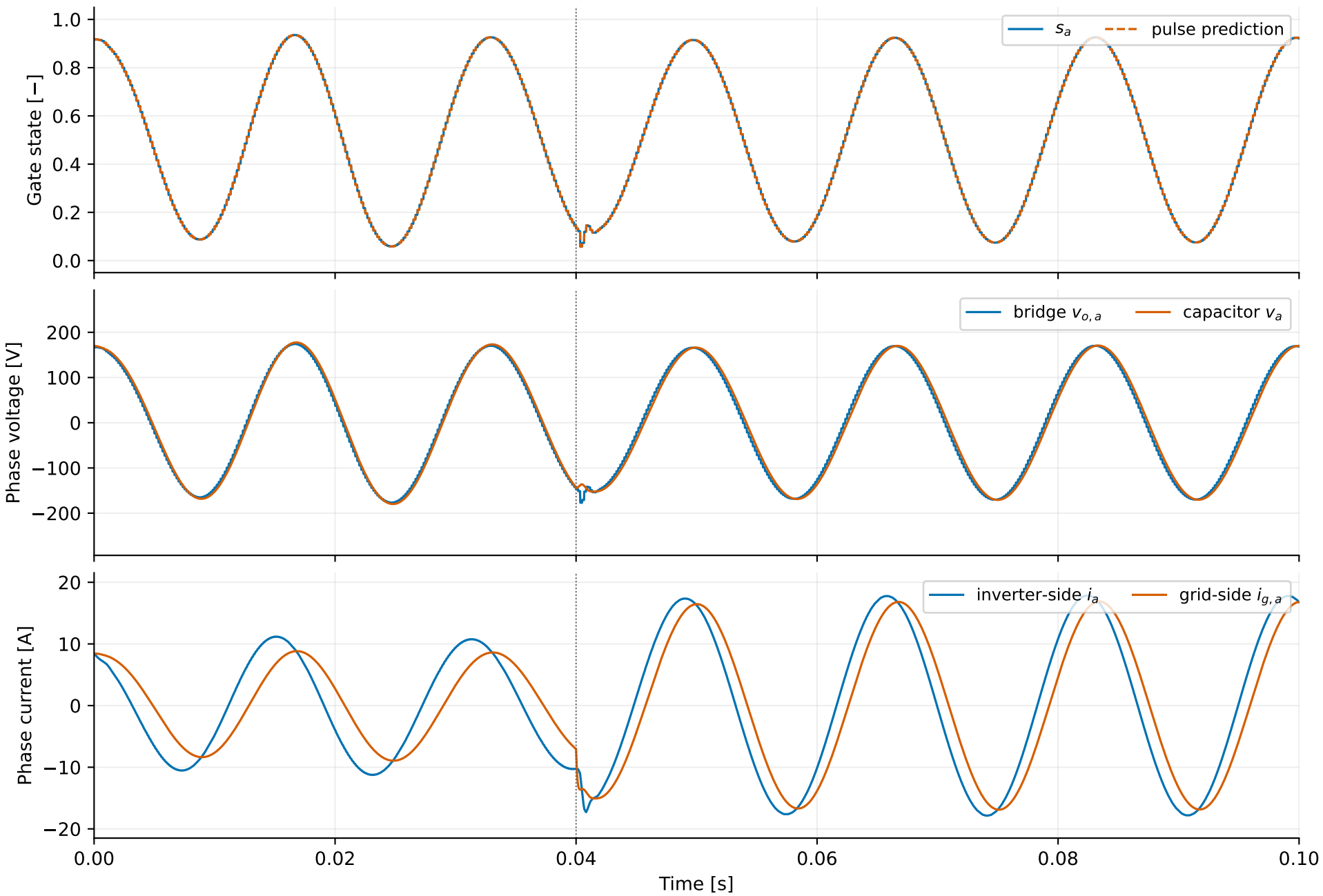
6000 Hz PWM, islanded voltage control, \mu = 240
