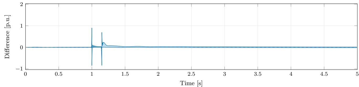
(c) EMT minus PhasorDynamics: range across channels
