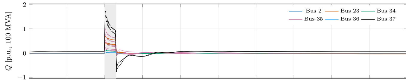
(b) GridKit PhasorDynamics; fault cleared at 1.15 s (30 machines)
