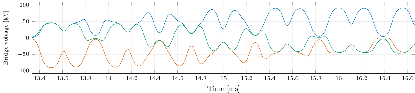
Plant 23.10: startup switching detail; \mu = 50000
