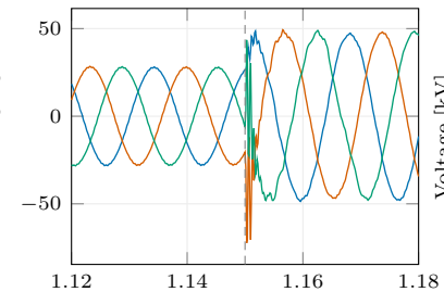
Bus 33; \mu = 50000
