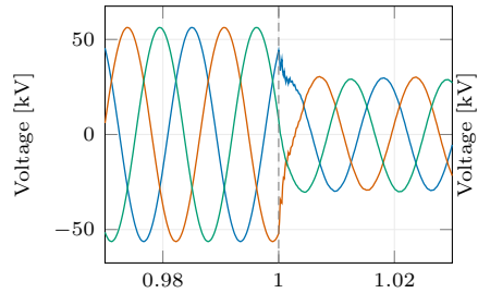
Bus 33; \mu = 50000
