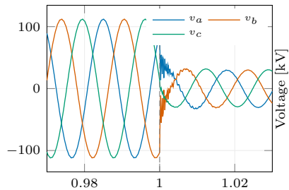
Bus 23; \mu = 50000
