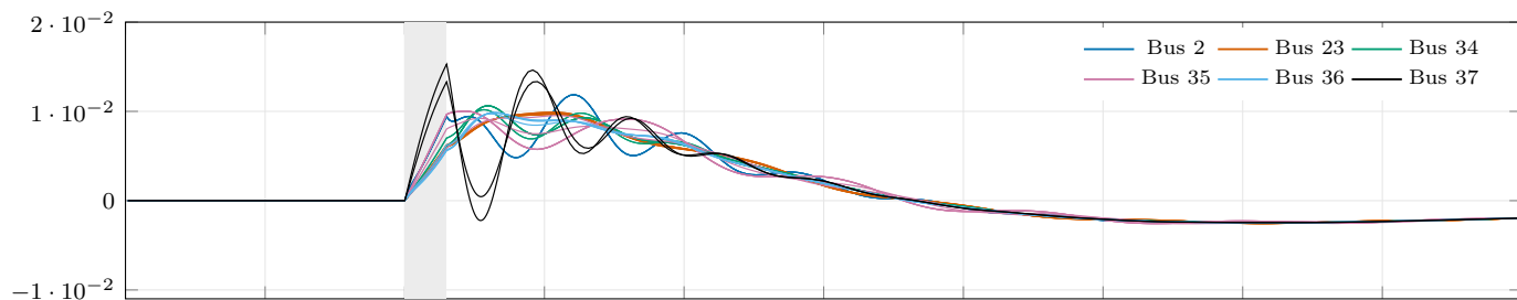
(c) EMT minus PhasorDynamics: range across channels
