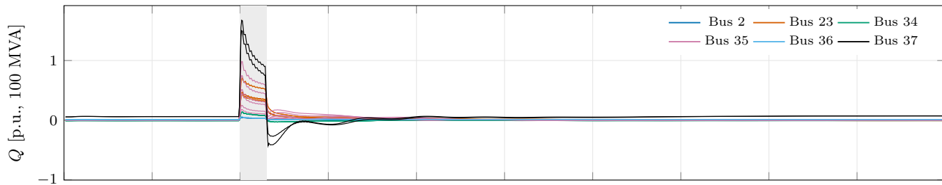
(b) GridKit PhasorDynamics; fault cleared at 1.15 s (30 machines)
