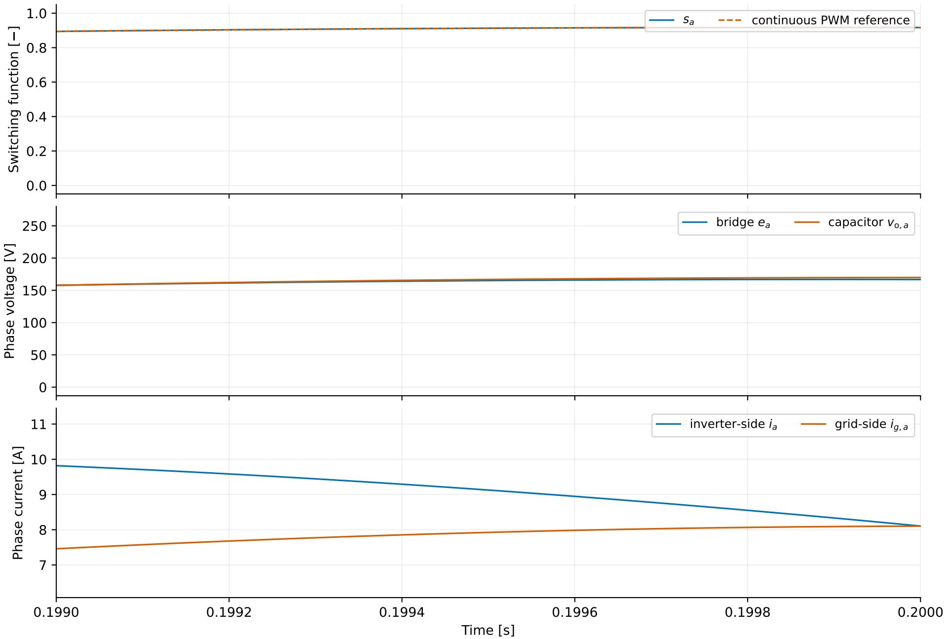
6000 Hz PWM, GFM, \mu = 240 \text{ s}^{-1}
